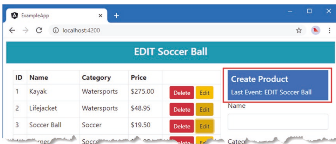
Figure 23-8. Filtering events
