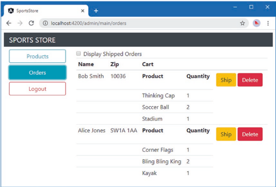
Figure 9-7. Managing orders
