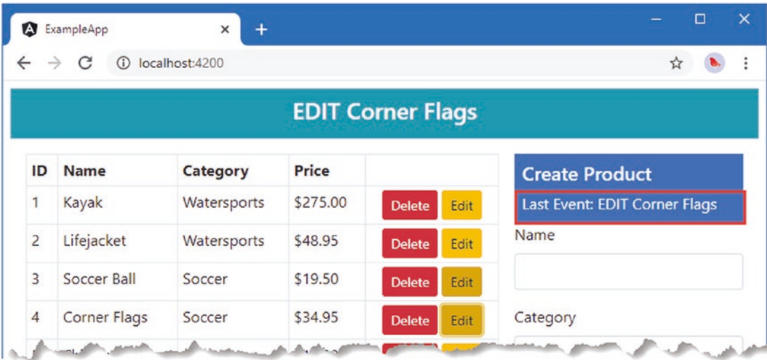
Figure 23-10. Skipping events
