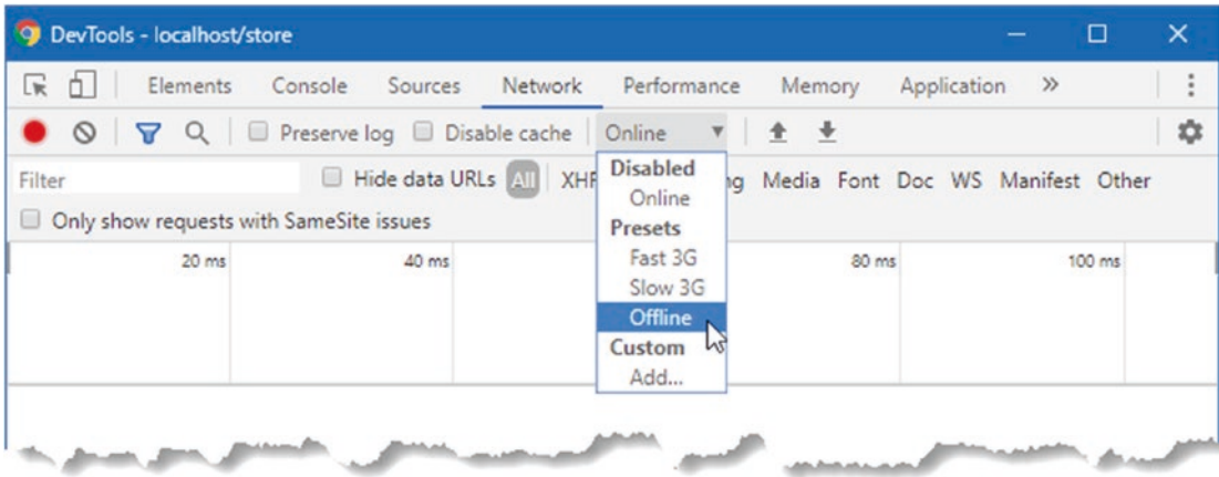
Figure 10-2. Going offline
