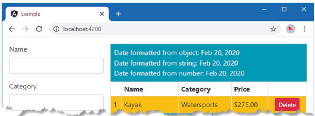
Figure 18-13. Formatting dates
