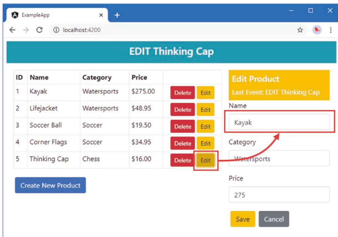
Figure 23-9. Transforming events
