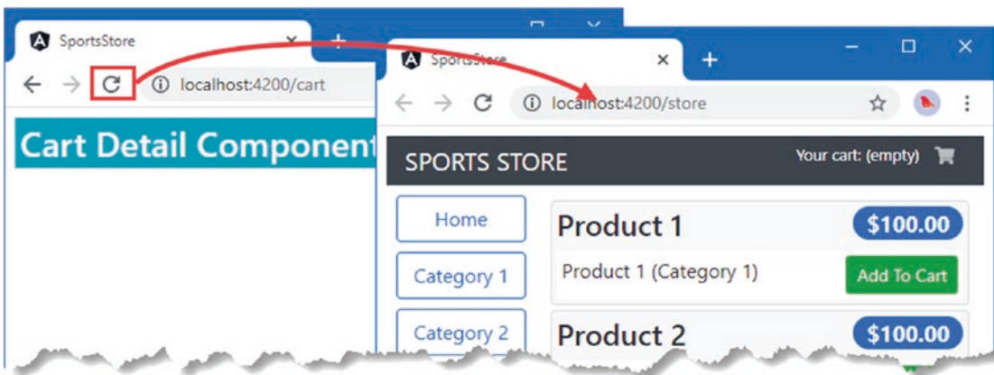
Figure 8-4. Guarding routes
