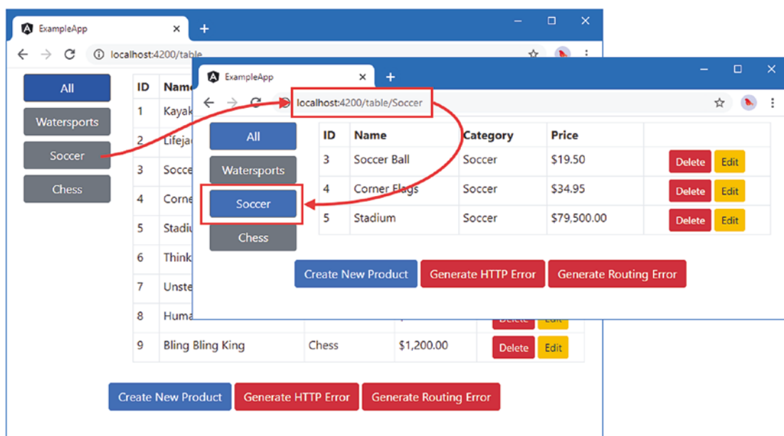
Figure 26-6. Filtering products
