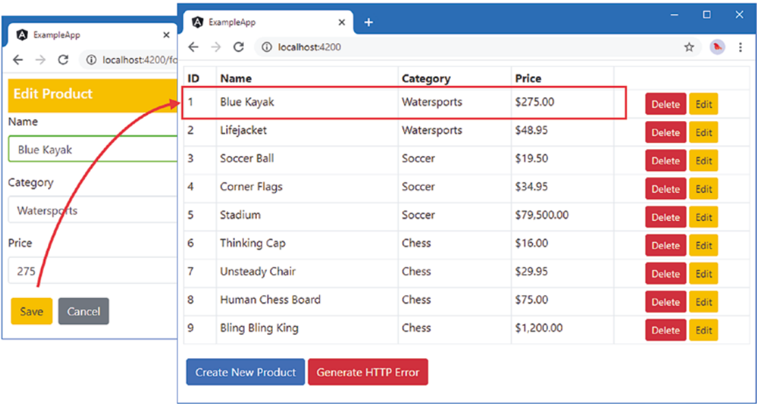
Figure 25-6. Navigating programmatically
